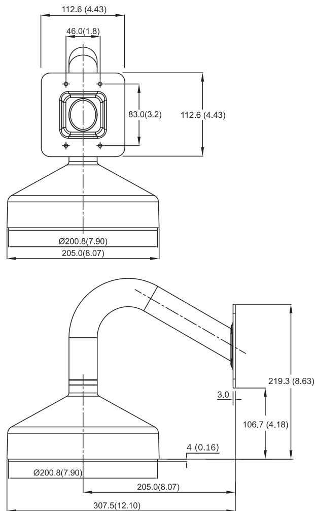
VDA-832FHD-WMT Wall mount dimensions
