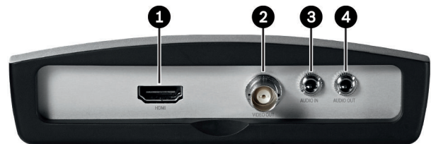
VIDEOJET decoder 3000 front view
