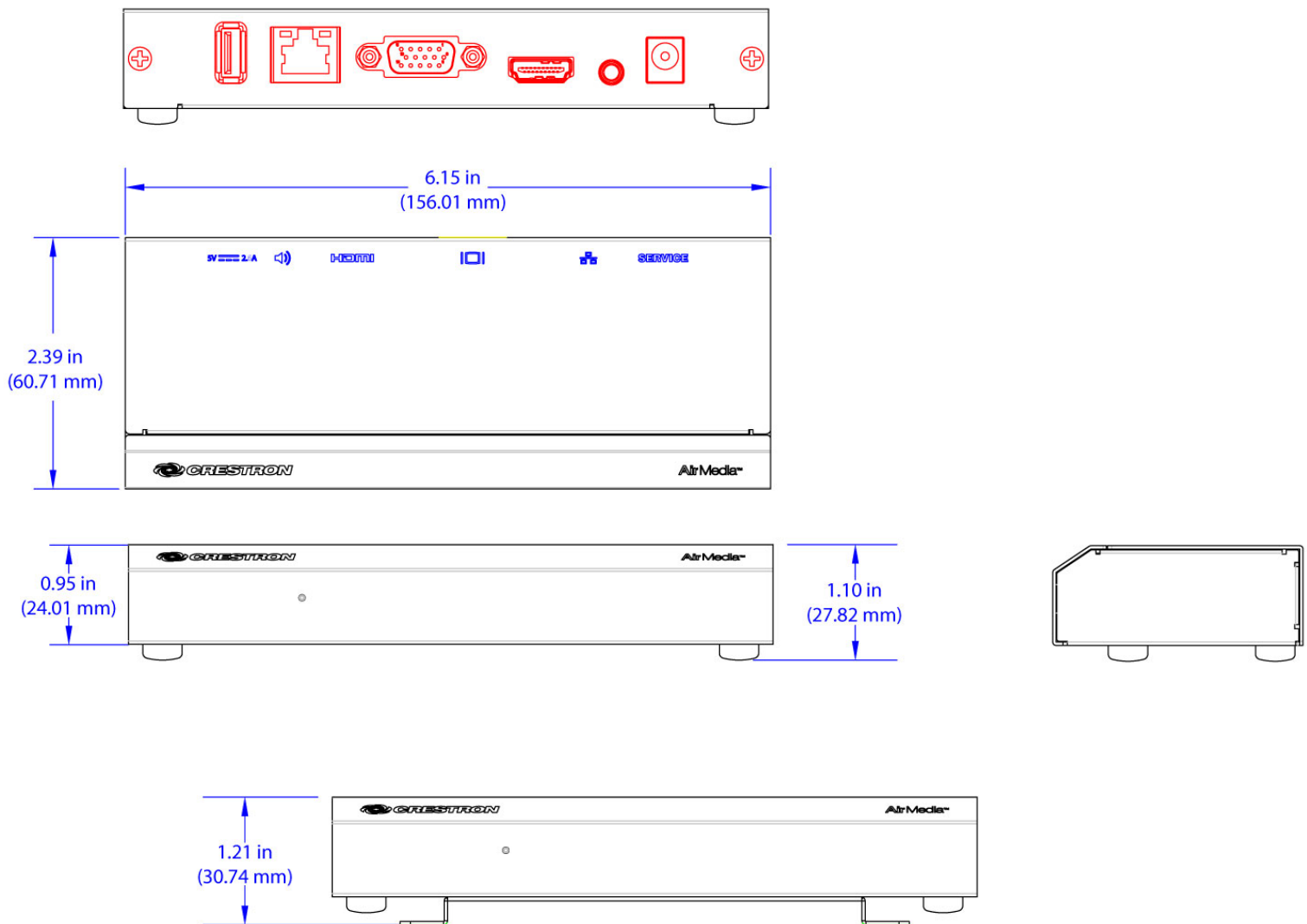
Shown with surface mount bracket attached
