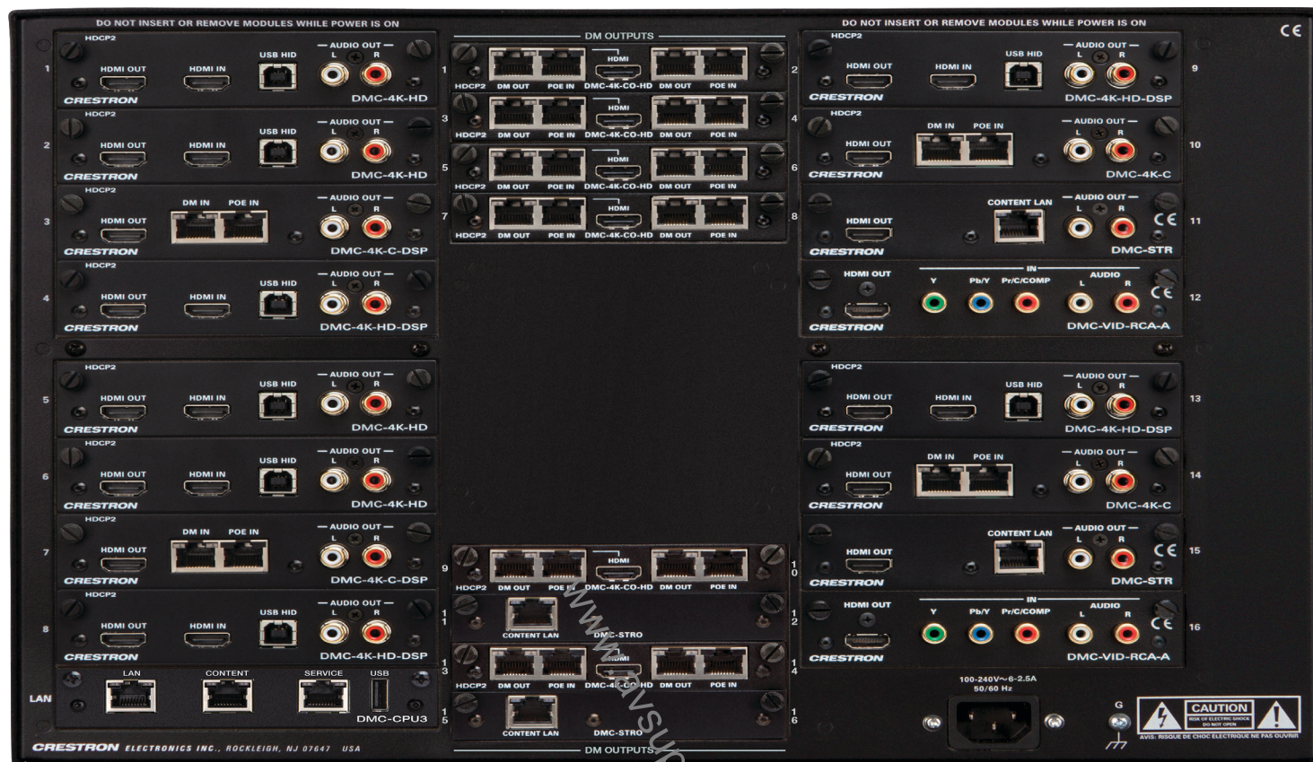
DM-MD16X16-CPU3 – Rear view with I/O cards installed
