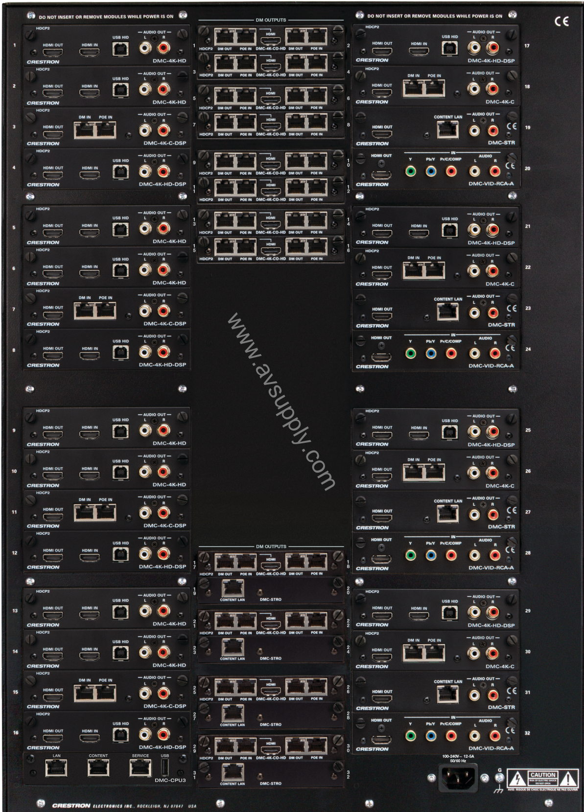
DM-MD32X32-CPU3-RPS – Rear view with I/O cards installed
