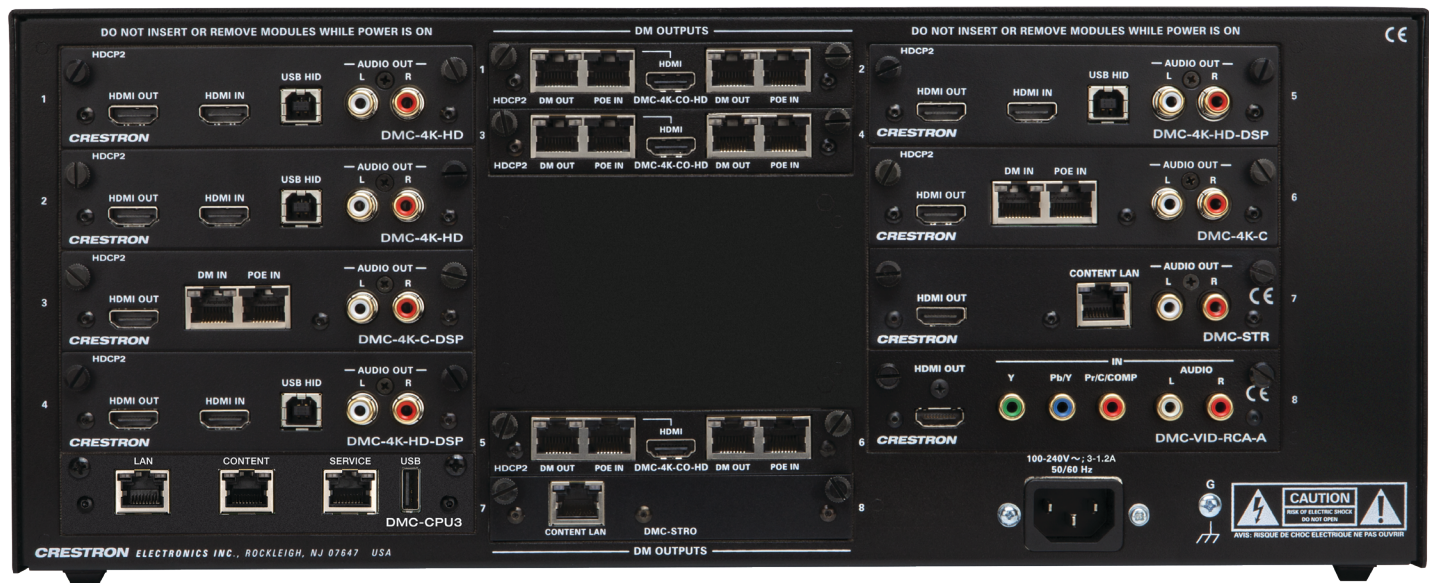
DM-MD8X8-CPU3 – Rear view with I/O cards installed
