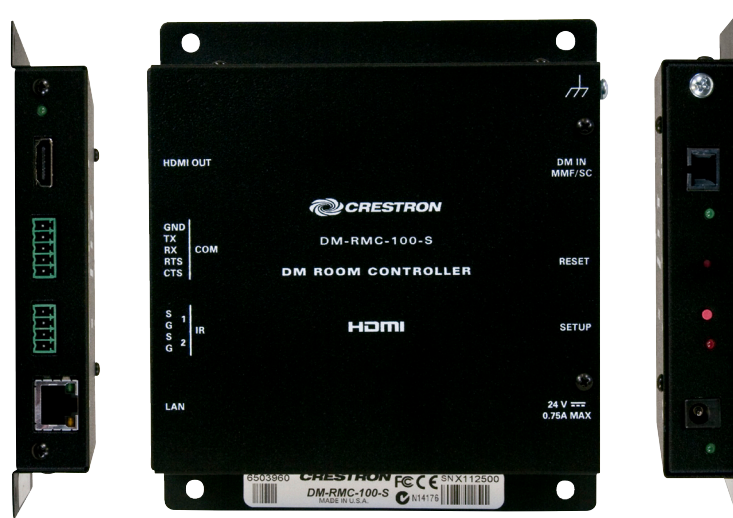
DM-RMC-100-S – Left, Front, and Right Views
