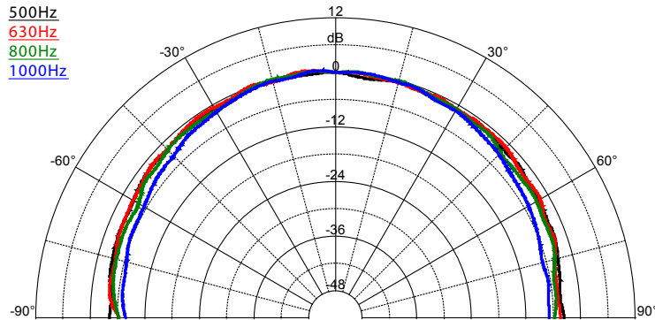
SAROS IC4T – Dispersion Pattern, 500 Hz - 1000 Hz
