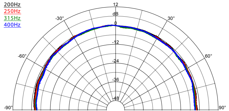
SAROS IC4T – Dispersion Pattern, 200 Hz - 400 Hz
