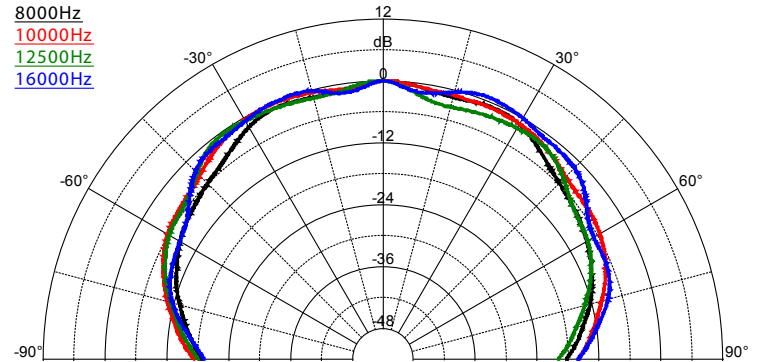
SAROS IC4T – Dispersion Pattern, 8000 Hz - 16000 Hz
