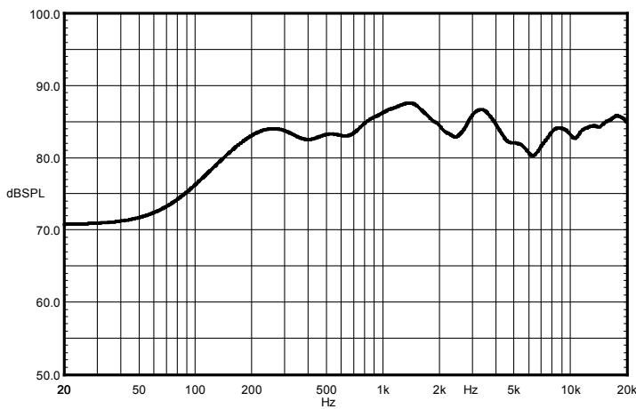
SAROS IC4T – Frequency Response
