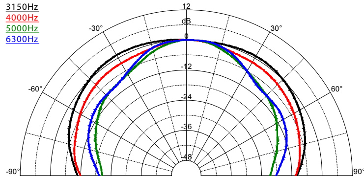
SAROS IC4T – Dispersion Pattern, 3150 Hz - 6300 Hz
