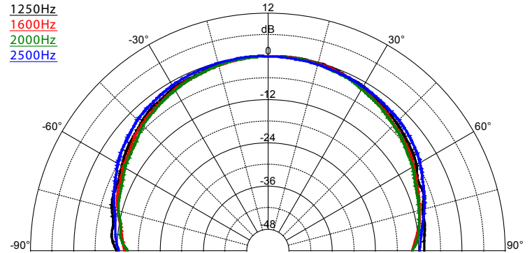
SAROS IC4T – Dispersion Pattern, 1250 Hz - 2500 Hz
