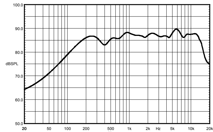
SAROS IC6T – Frequency Response
