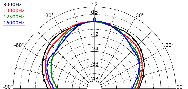
SAROS SR4T – Dispersion Pattern, 8000 Hz - 16000 Hz
