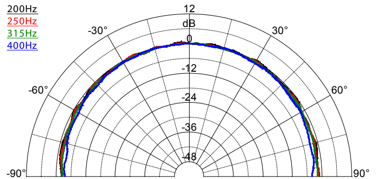
SAROS SR4T – Dispersion Pattern, 200 Hz - 400 Hz
