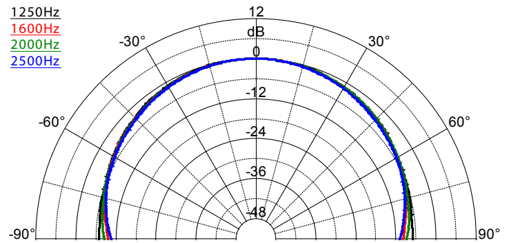
SAROS SR4T – Dispersion Pattern, 1250 Hz - 2500 Hz
