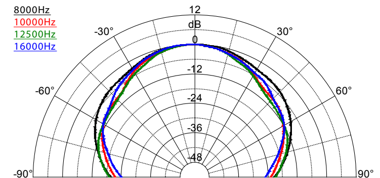
SAROS SR6T – Dispersion Pattern, 8000 Hz - 16000 Hz
