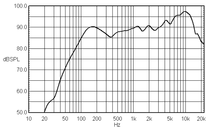
SAROS SR6T – Frequency Response
