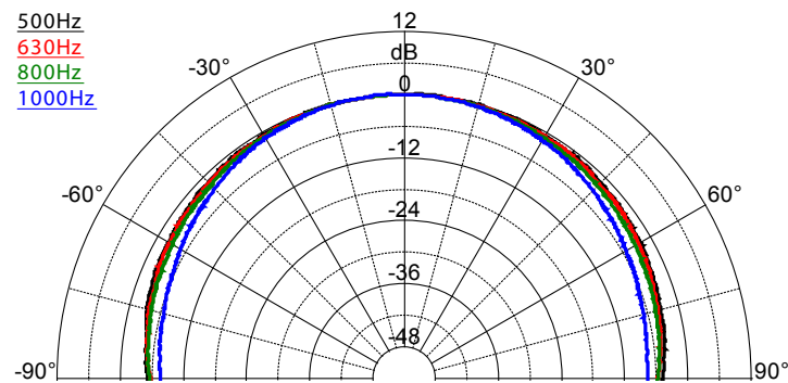
SAROS SR6T – Dispersion Pattern, 500 Hz - 1000 Hz
