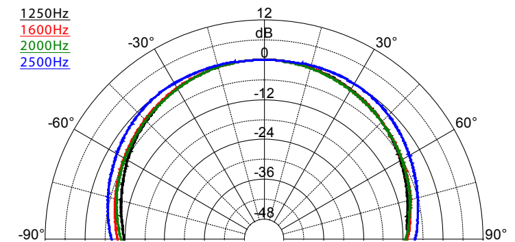
SAROS SR6T – Dispersion Pattern, 1250 Hz - 2500 Hz
