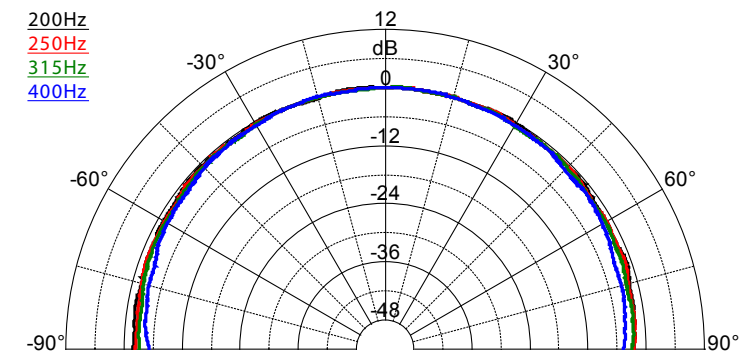
SAROS SR6T – Dispersion Pattern, 200 Hz - 400 Hz
