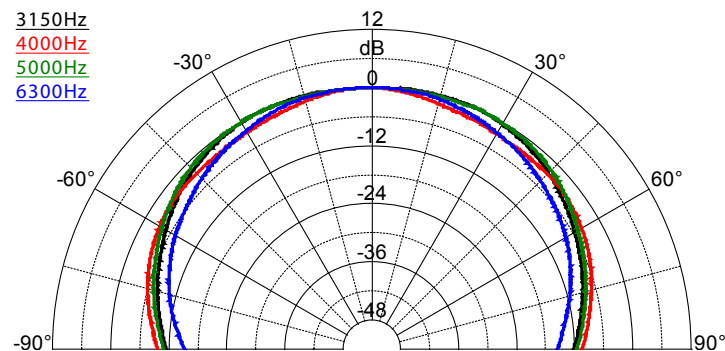
SAROS SR6T – Dispersion Pattern, 3150 Hz - 6300 Hz
