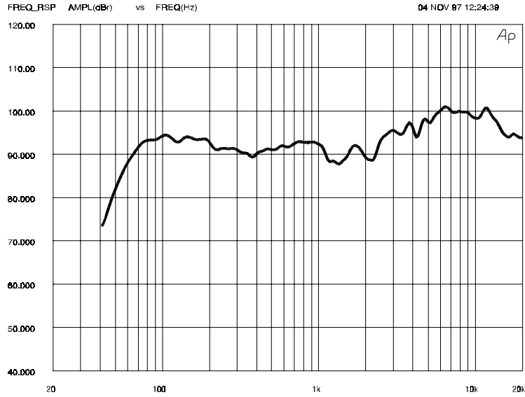
Figure 1 — EVI-28 Long-Throw Frequency Response (4 volts/10 feet normalized to 1 watt/ 1 meter, anechoic environment)
