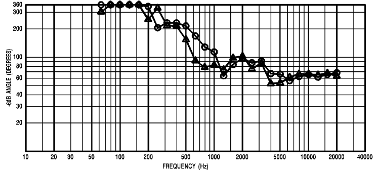
Figure 6 — EVI-28 Long-Throw Horizontal and Vertical Beamwidth vs. Frequency (anechoic environment @ 20ft)
