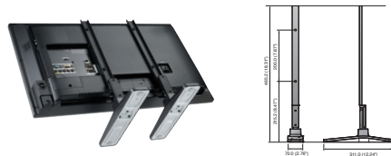
Foot Stand SBM-320ST
