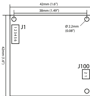
J1 USB Out
